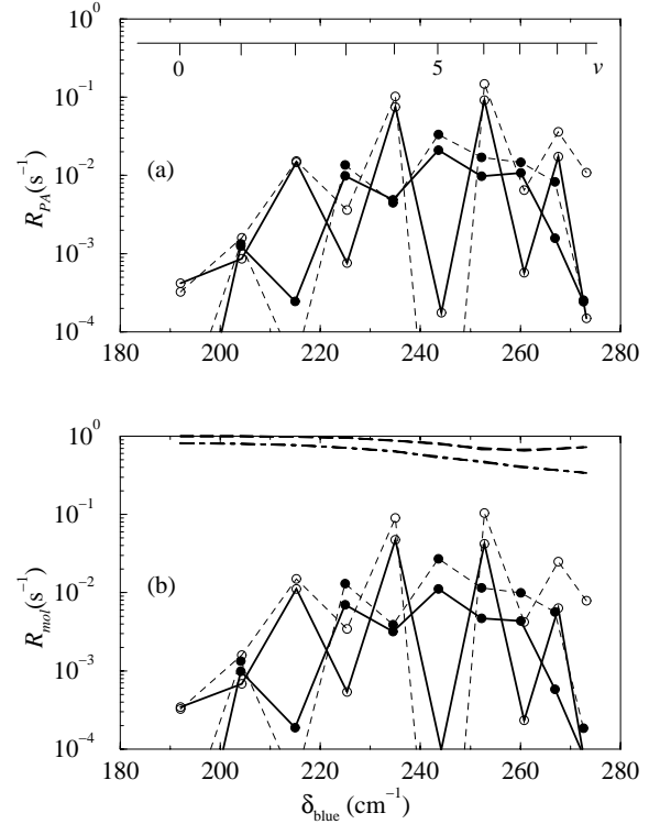
Fig. 5. (a) Photoassociation rate per atom \mathcal{R}_{\text{PA}} and (b) cold molecule formation rate per atom \mathcal{R}_{\text{mol}} , as a function of the detuning \delta_{\text{blue}} of the PA laser, for the external well of the 0_g^+(P_{3/2}) state. 0_g^+ levels up to v = 9 are considered. Typical experimental conditions of a Rb magneto-optical trap are assumed, i.e. I = 10 \text{ W/cm}^2 , n_{\text{at}} = 3 \times 10^{10} \text{ cm}^{-3} , T = 120 \mu\text{K} . Both isotopes 85 Rb (open circles) and 87 Rb (closed circles) are considered. Calculations without (dashed lines) and with (solid lines) inclusion of a variable transition dipole moment are displayed. In panel (b) the sum of Franck-Condon factors involved in equations (8, 9), without (long dashed line) and with (dot-dashed line) inclusion of a variable transition dipole moment, are shown on the same scale.
